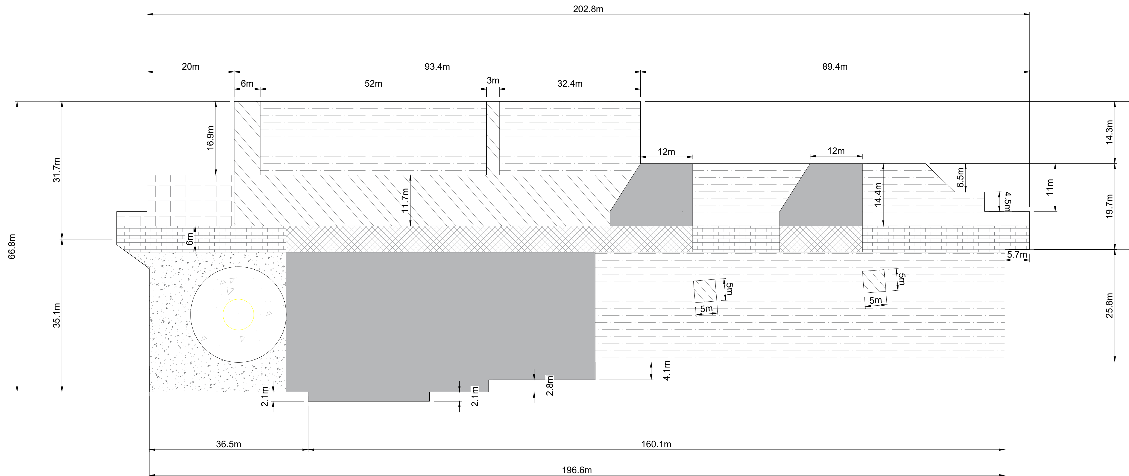
CRANE HARDSTAND - PLAN SCALE 1:500
